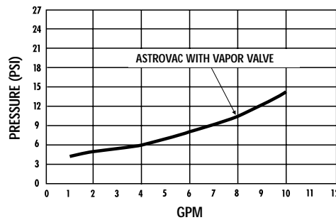
FLOW RATE VS. INLET PRESSURE
